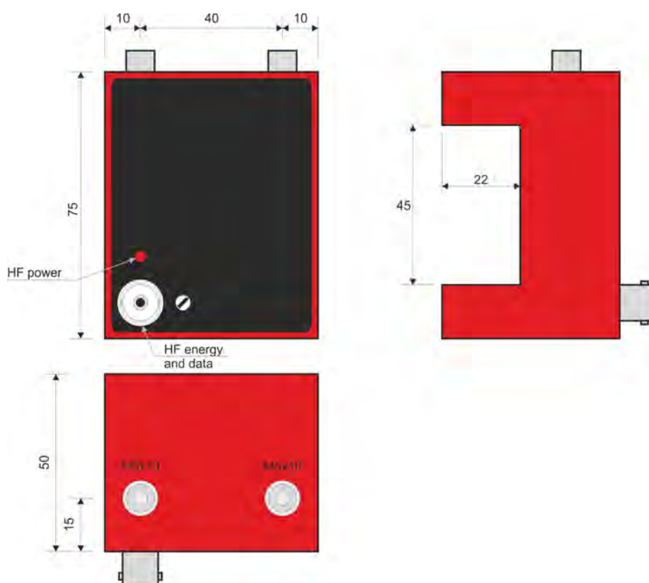
Fig. 4: Stator antenna A9e_PCM
