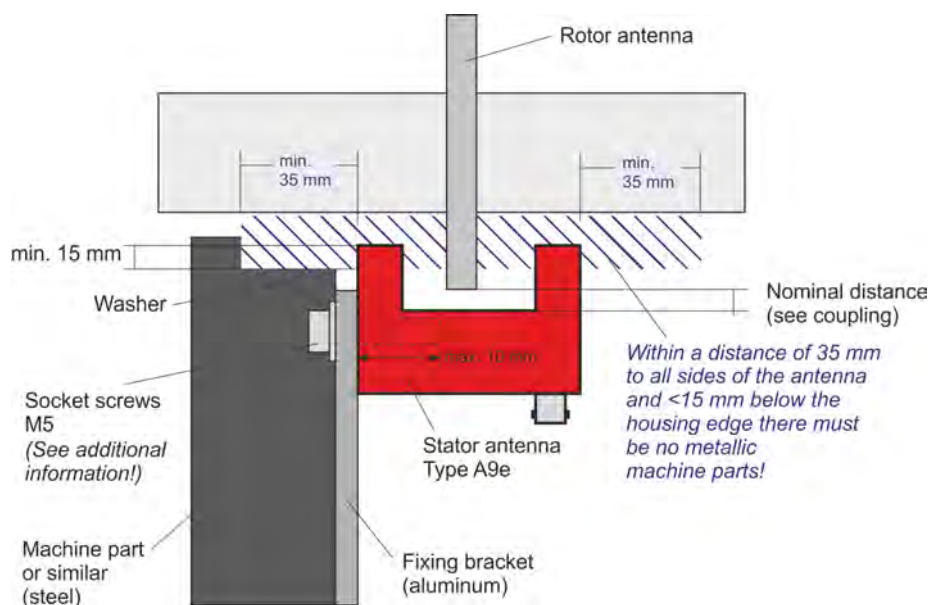
Fig. 6: Minimum distance antenna A9e
