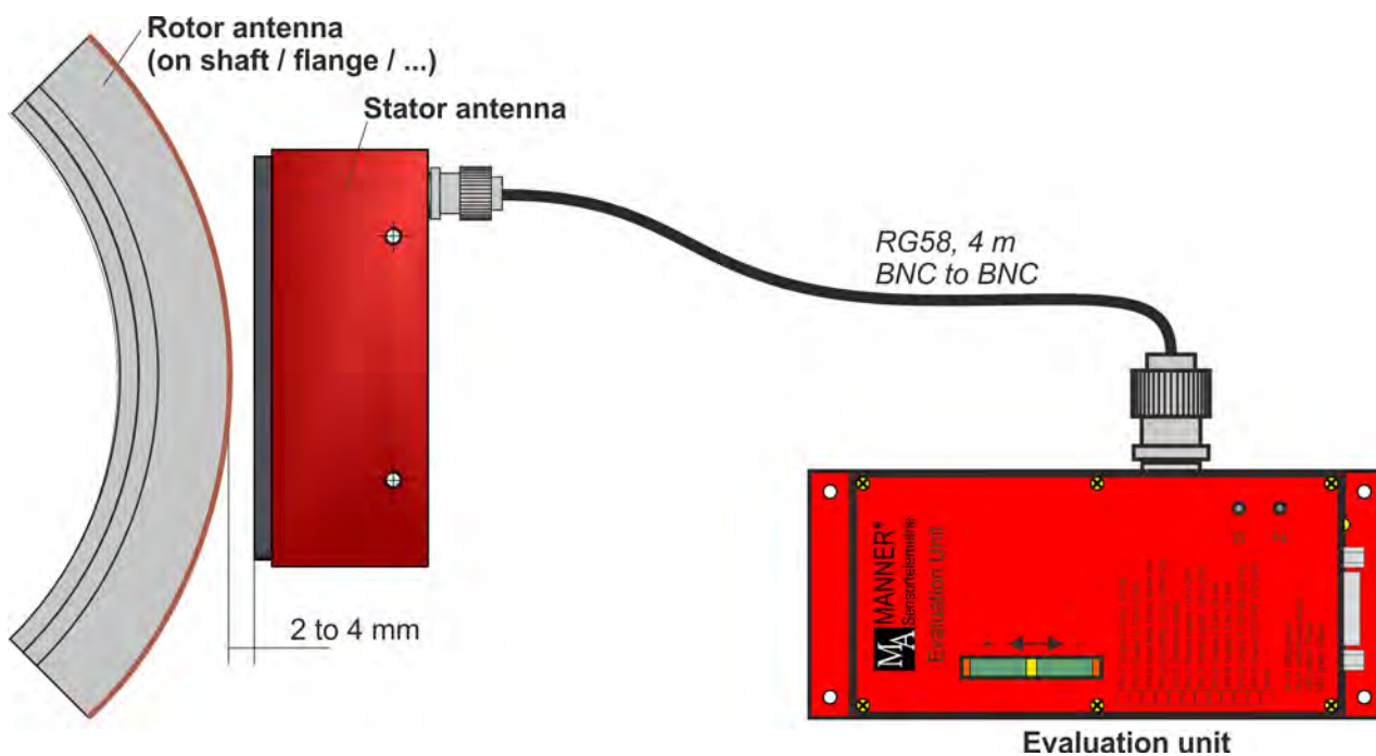
Fig. 5: Coupling
