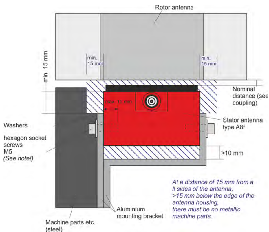
Fig. 6: Minimum distance antenna A8f
