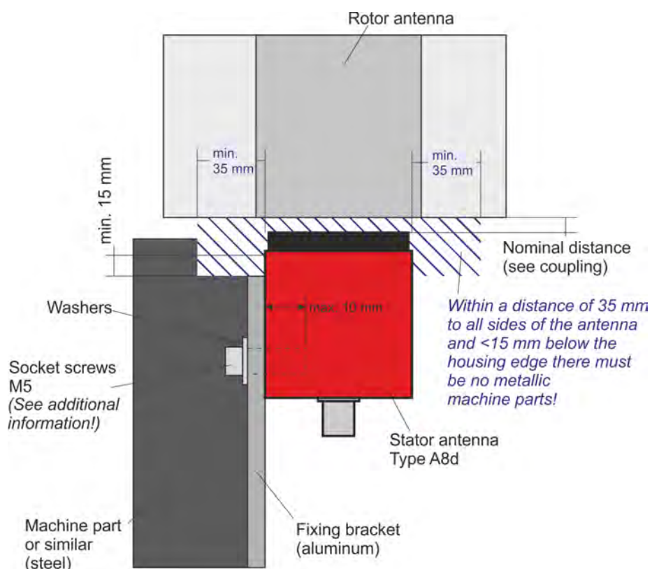
Fig. 6: Minimum distance antenna A8d
