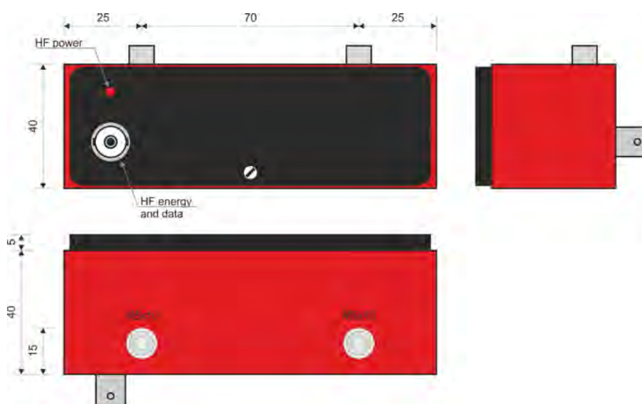
Fig. 4: Stator antenna A8d_PCM
