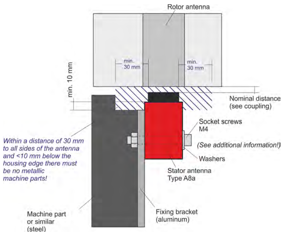
Fig. 6: Minimum distance antenna A8a
